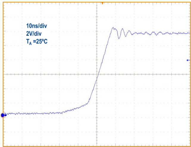
Figure 7 SW Output Rise Time
