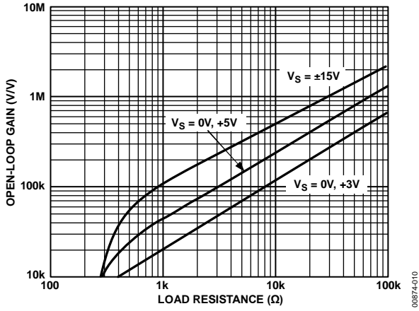
Figure 10. Open-Loop Gain vs. Load Resistance
