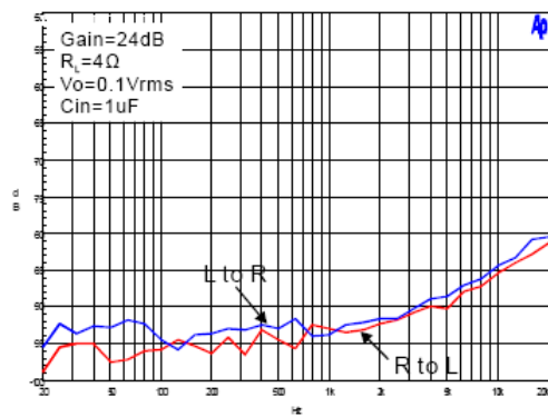
6. Crosstalk
