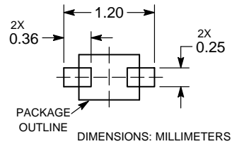
DIMENSIONS: MILLIMETERS
