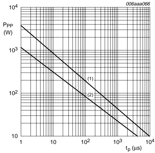
T_{amb} = 25\text{ }^\circ\text{C} t_p = 8/20\text{ }\mu s exponential decay waveform; see Figure 1 (1) PESD3V3L1BA and PESD5V0L1BA (2) PESD12VL1BA; PESD15VL1BA; PESD24VL1BA
