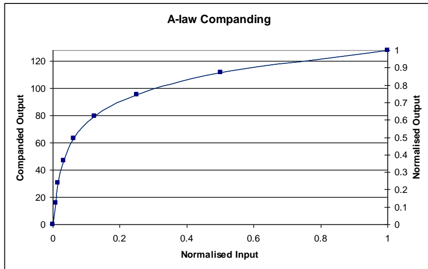
Figure 64 A-Law Companding
