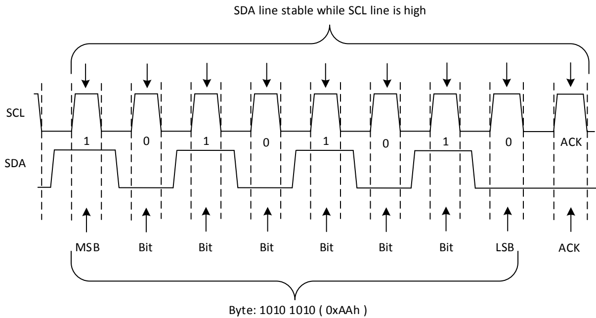
Figure 7-4. Bit Transfer
