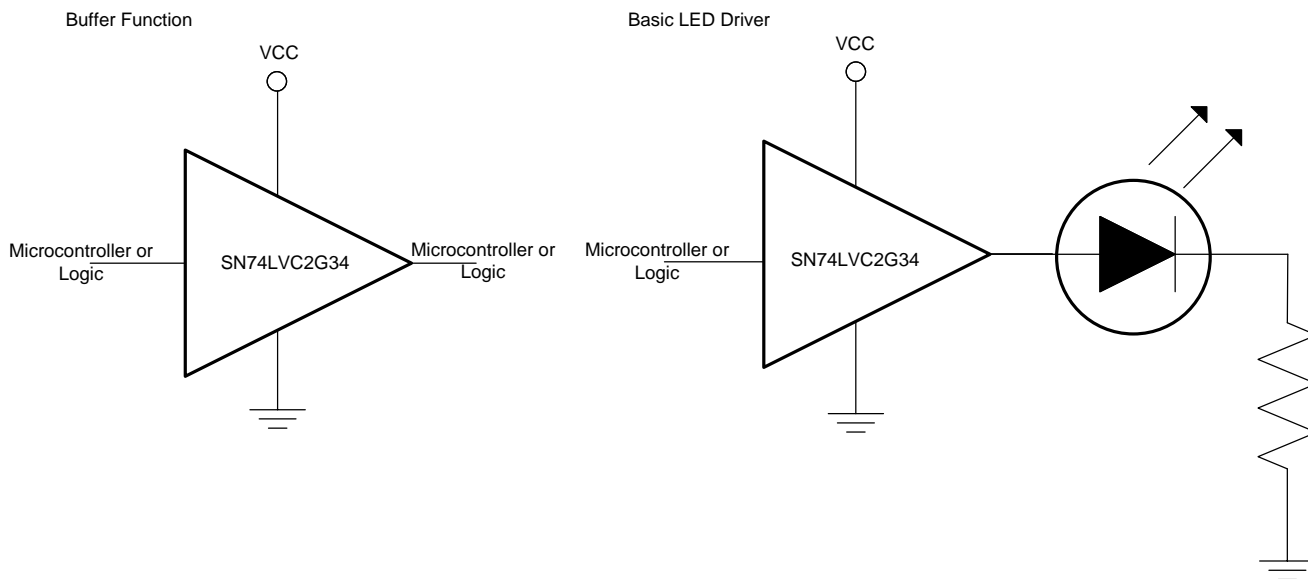
Figure 3. Typical Application
