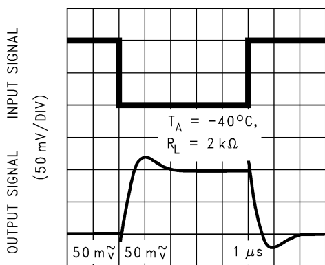
TIME (1 μs/DIV) Figure 43. Inverting Small Signal Pulse Response
