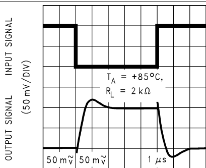
TIME (1 μs/DIV) Figure 45. Inverting Small Signal Pulse Response
