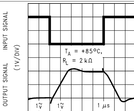
TIME (1 μs/DIV) Figure 46. Inverting Large Signal Pulse Response
