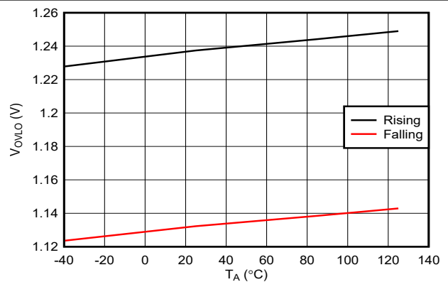
Figure 6-18. OVLO Pin Threshold vs Temperature
