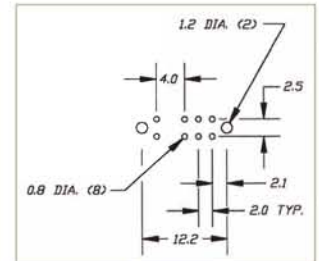
P.C. MOUNTING
