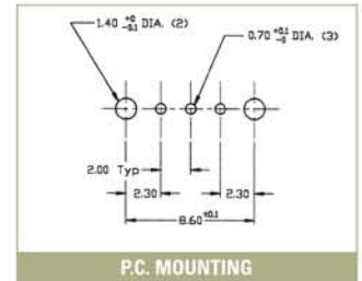
P.C. MOUNTING
