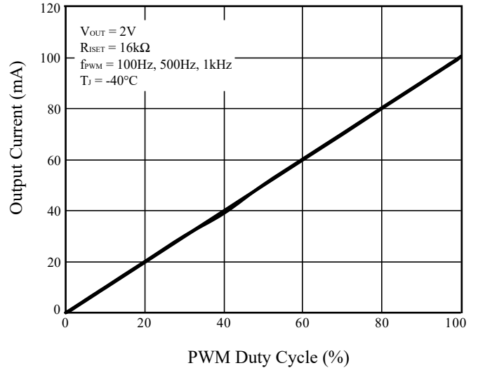
Figure 36 Output Current vs. PWM Duty Cycle
