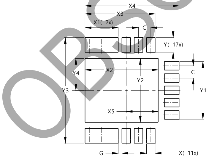
V-QFN4040-17
